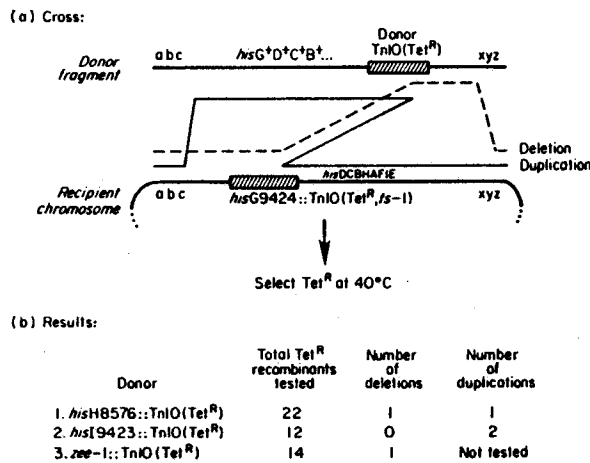
FIG. 9. Isolation of duplications and deletions with specified endpoints using a Tn10 ( tet R -ts ) recipient.
