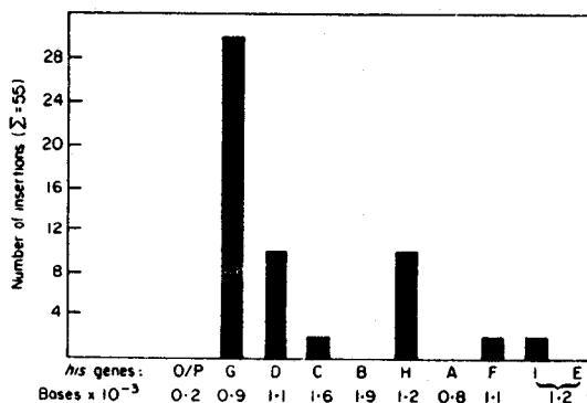
FIG. 1. Distribution of Tn10 insertions in the Salmonella histidine operon. 55 independent his::Tn10 insertion auxotrophs were isolated following infection of S. typhimurium LT2 with a suitable Tn10 vehicle (see section 4). The positions of these insertions within the his operon were determined by deletion mapping and complementation tests as described elsewhere (Kleckner et al. , 1975).
